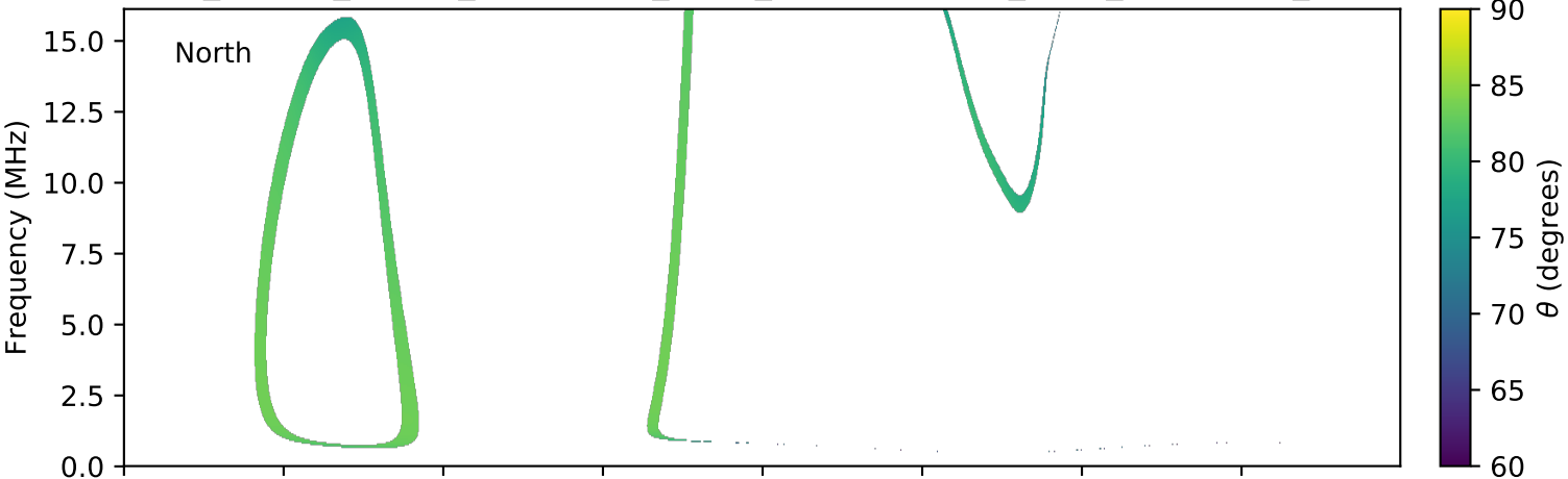
expres_cassini_jupiter_ganymede_isaac_lossc-wid1deg_3kev_20000311_v01.cdf
