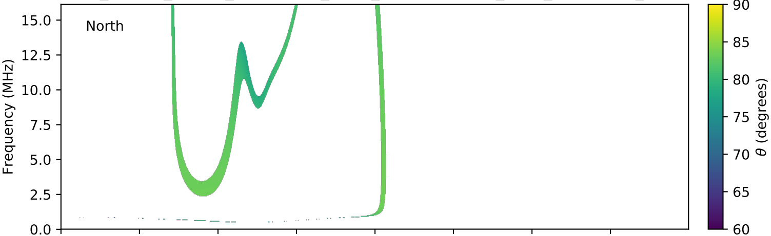
expres_cassini_jupiter_ganymede_isaac_lossc-wid1deg_3kev_20000307_v01.cdf
