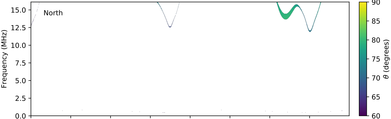
expres_cassini_jupiter_ganymede_isaac_lossc-wid1deg_3kev_20000306_v01.cdf
