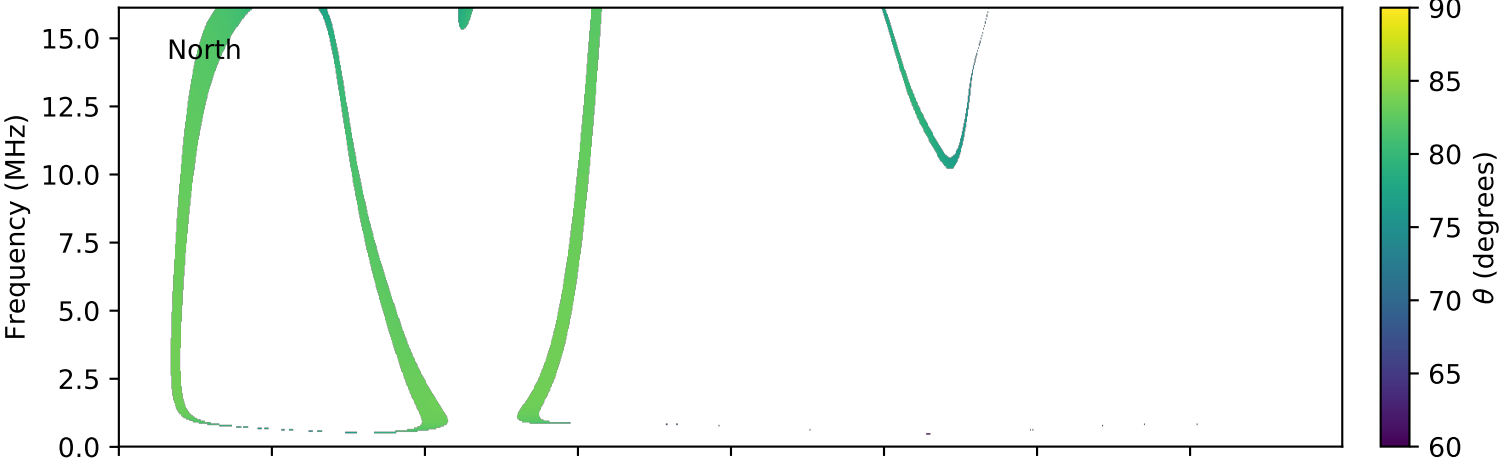
expres_cassini_jupiter_ganymede_isaac_lossc-wid1deg_3kev_20000304_v01.cdf
