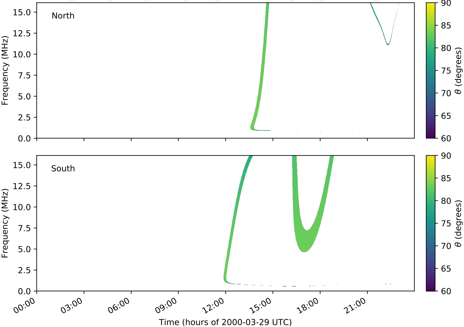
expres_cassini_jupiter_europa_isaac_lossc-wid1deg_3kev_20000329_v01.cdf
