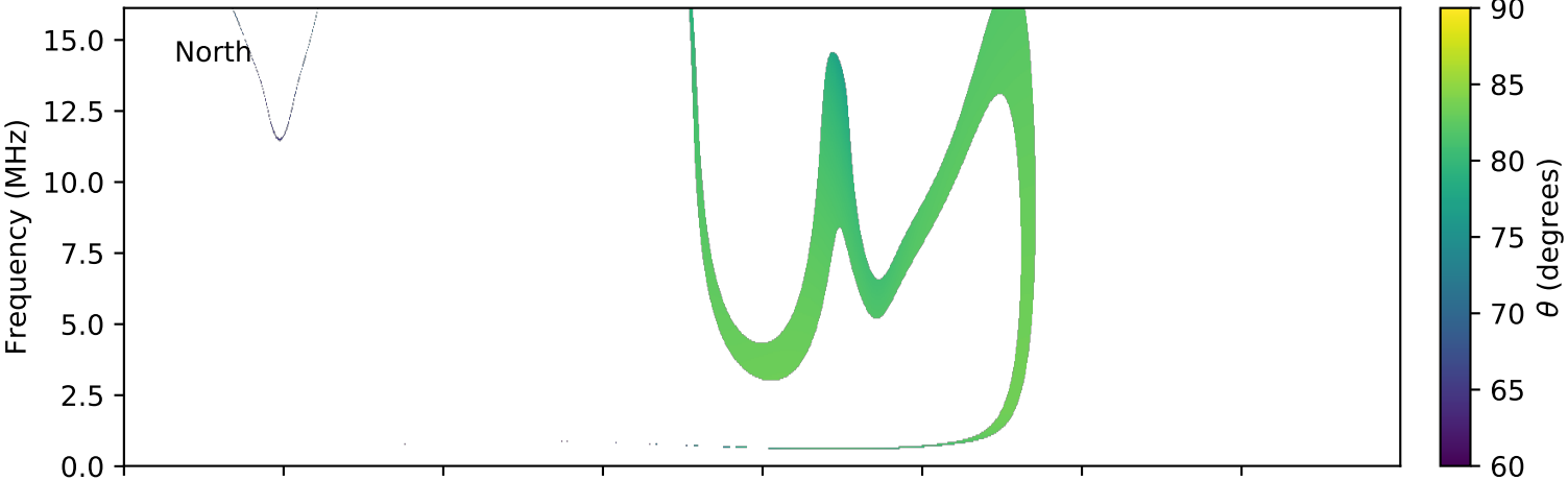
expres_cassini_jupiter_europa_isaac_lossc-wid1deg_3kev_20000327_v01.cdf
