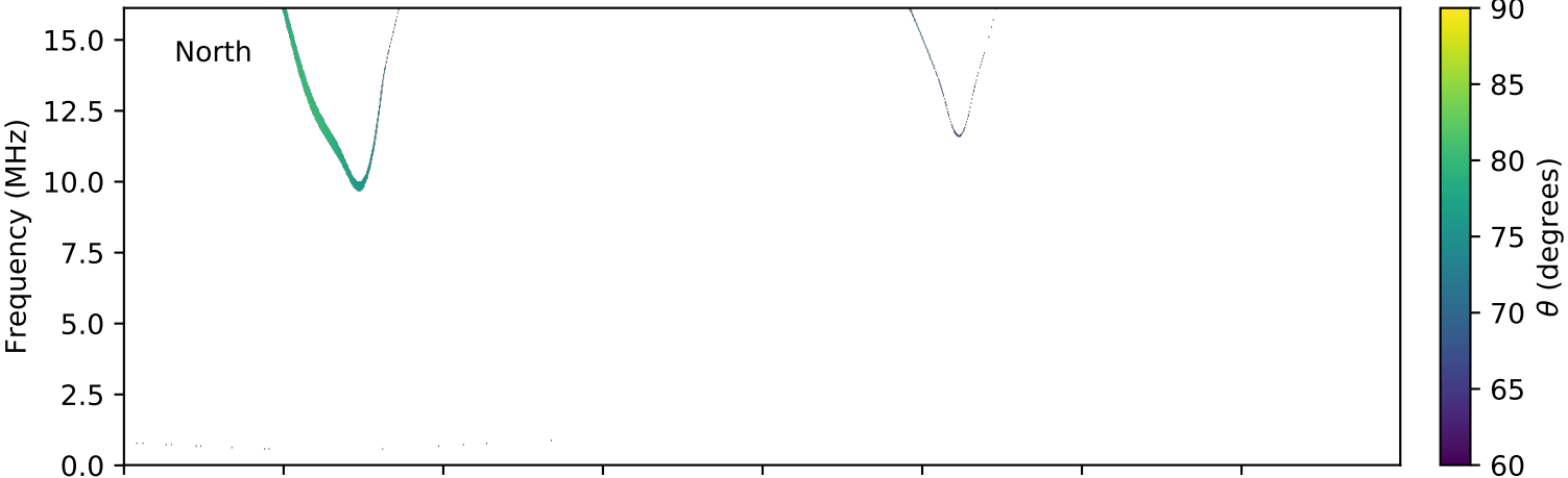
expres_cassini_jupiter_europa_isaac_lossc-wid1deg_3kev_20000326_v01.cdf
