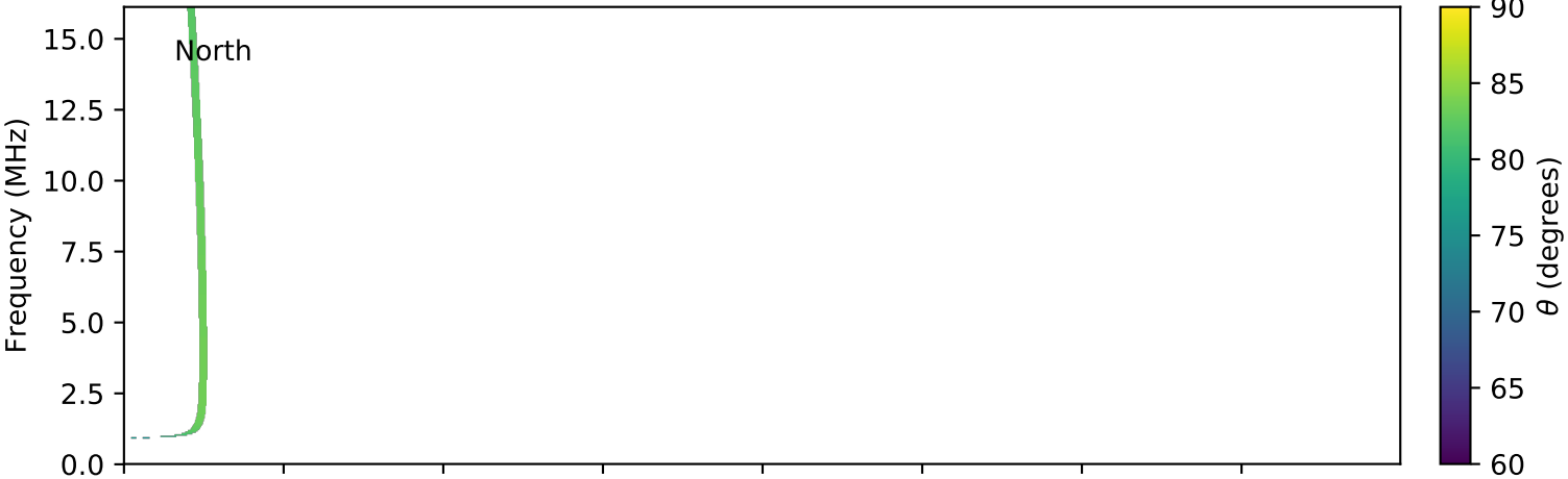
expres_cassini_jupiter_europa_isaac_lossc-wid1deg_3kev_20000324_v01.cdf
