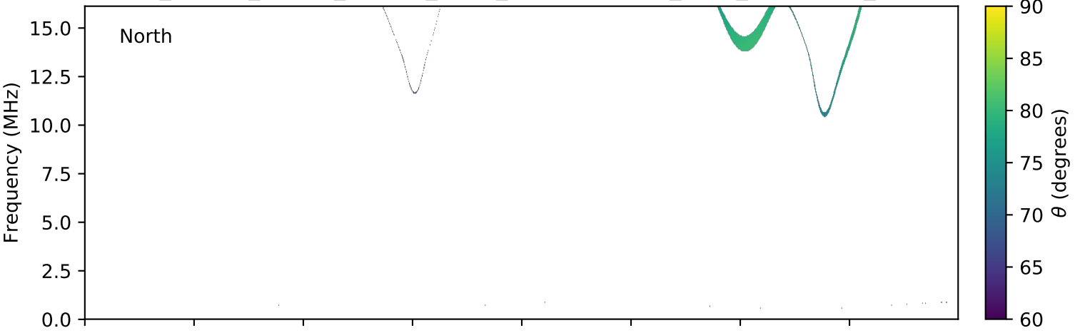
expres_cassini_jupiter_europa_isaac_lossc-wid1deg_3kev_20000323_v01.cdf
