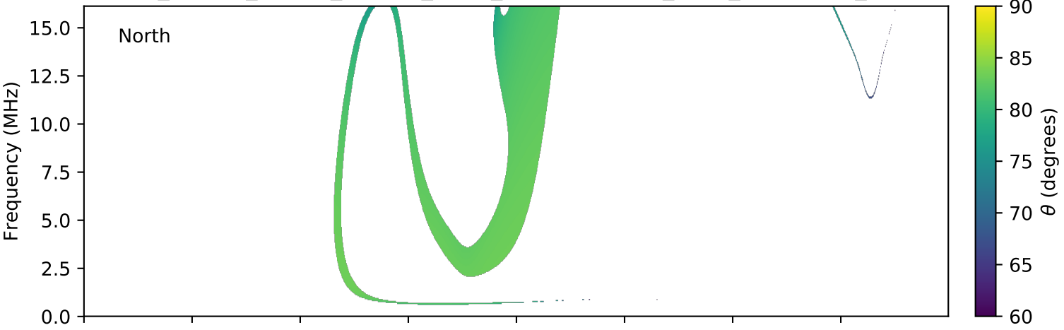
expres_cassini_jupiter_europa_isaac_lossc-wid1deg_3kev_20000322_v01.cdf
