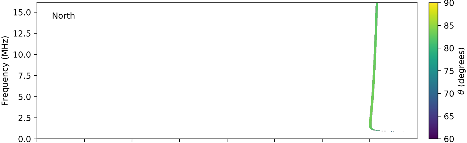
expres_cassini_jupiter_europa_isaac_lossc-wid1deg_3kev_20000318_v01.cdf
