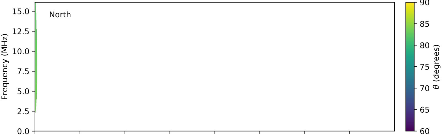
expres_cassini_jupiter_europa_isaac_lossc-wid1deg_3kev_20000317_v01.cdf
