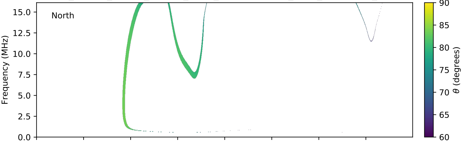
expres_cassini_jupiter_europa_isaac_lossc-wid1deg_3kev_20000315_v01.cdf
