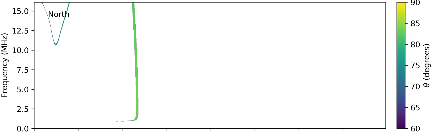
expres_cassini_jupiter_europa_isaac_lossc-wid1deg_3kev_20000306_v01.cdf
