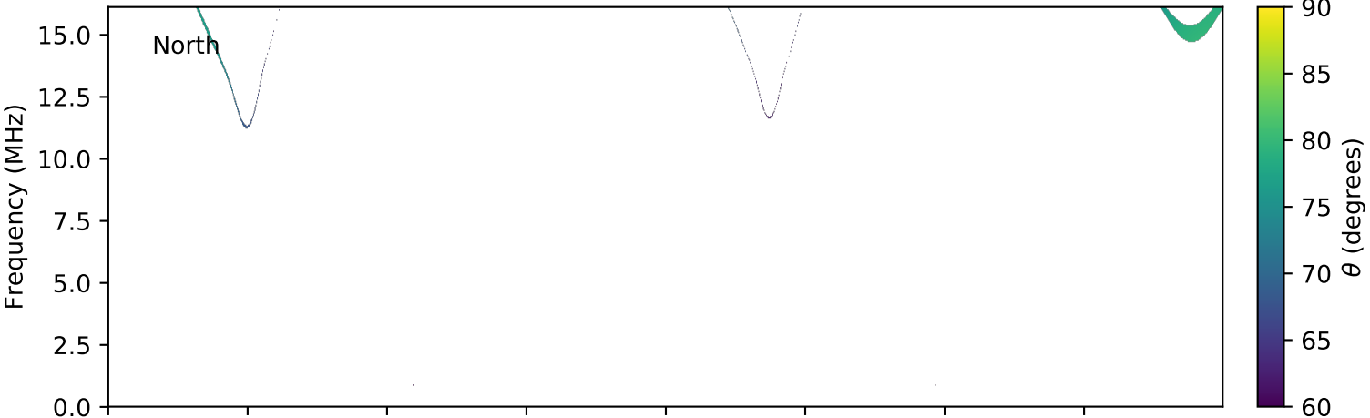
expres_cassini_jupiter_europa_isaac_lossc-wid1deg_3kev_20000305_v01.cdf
