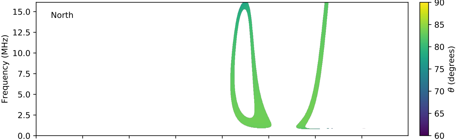
expres_cassini_jupiter_europa_isaac_lossc-wid1deg_3kev_20000304_v01.cdf
