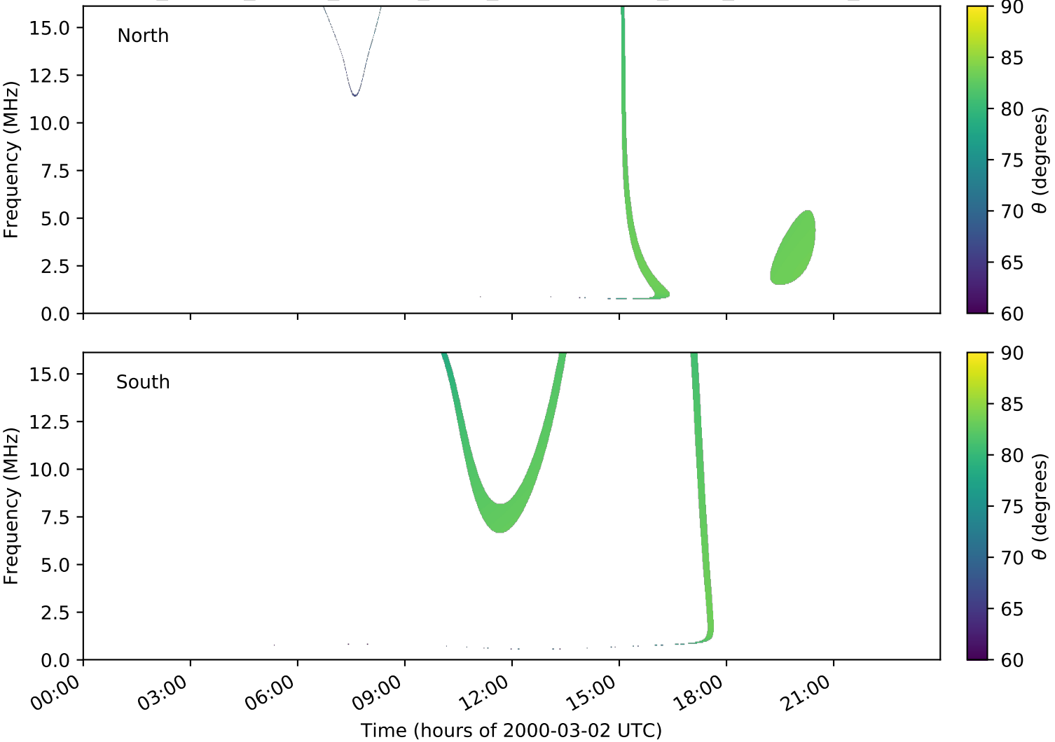
expres_cassini_jupiter_europa_isaac_lossc-wid1deg_3kev_20000302_v01.cdf
