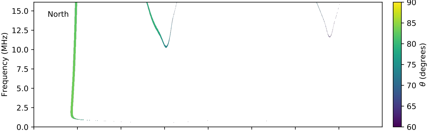
expres_cassini_jupiter_europa_isaac_lossc-wid1deg_3kev_20000301_v01.cdf
