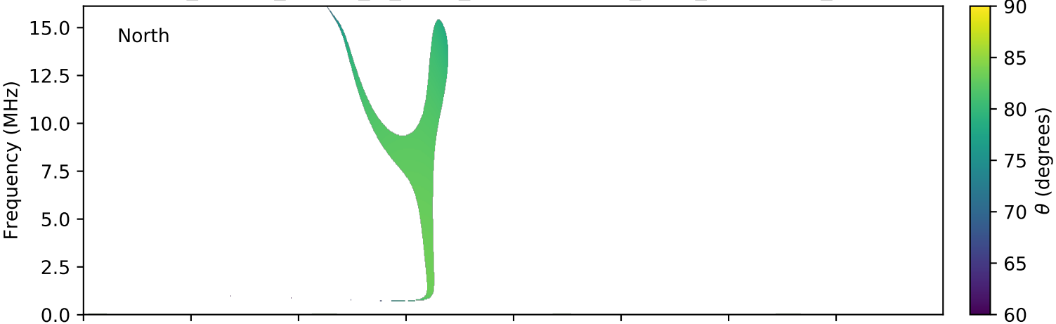
expres_cassini_jupiter_io_isaac_lossc-wid1deg_3kev_20000221_v01.cdf
