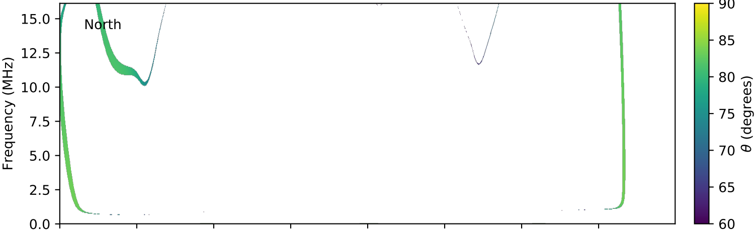
expres_cassini_jupiter_io_isaac_lossc-wid1deg_3kev_20000217_v01.cdf
