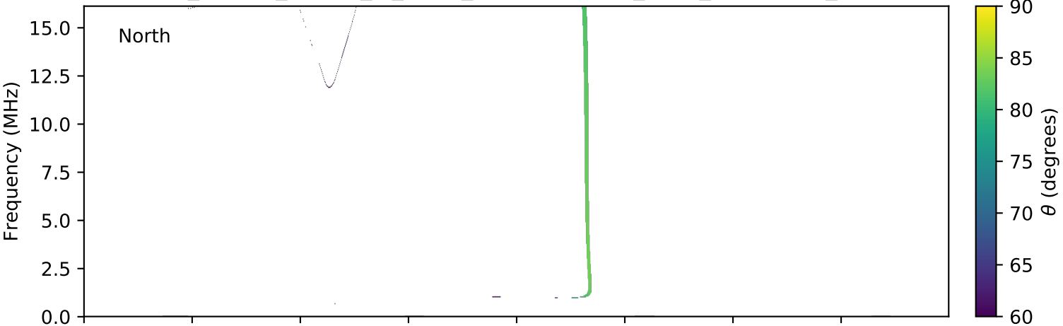
expres_cassini_jupiter_io_isaac_lossc-wid1deg_3kev_20000212_v01.cdf
