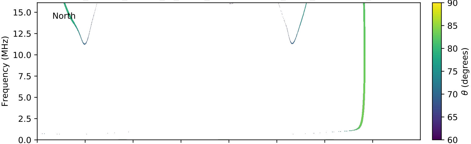
expres_cassini_jupiter_io_isaac_lossc-wid1deg_3kev_20000210_v01.cdf
