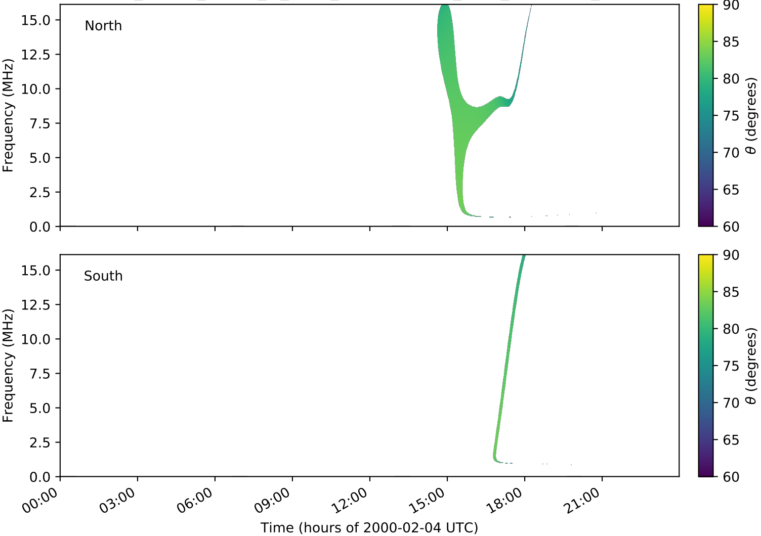
expres_cassini_jupiter_io_isaac_lossc-wid1deg_3kev_20000204_v01.cdf
