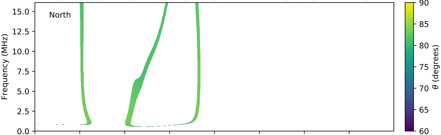
expres_cassini_jupiter_ganymede_isaac_lossc-wid1deg_3kev_20000229_v01.cdf
