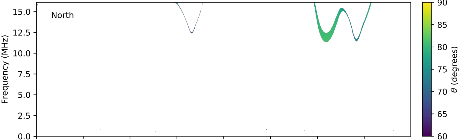
expres_cassini_jupiter_ganymede_isaac_lossc-wid1deg_3kev_20000228_v01.cdf
