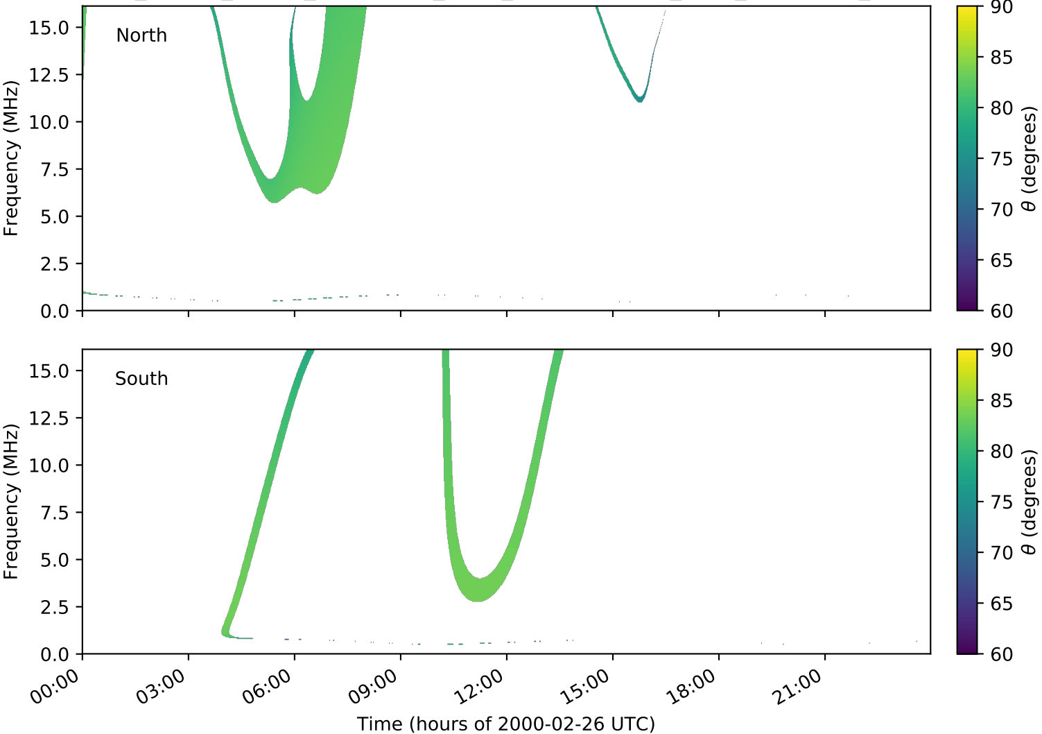
expres_cassini_jupiter_ganymede_isaac_lossc-wid1deg_3kev_20000226_v01.cdf
