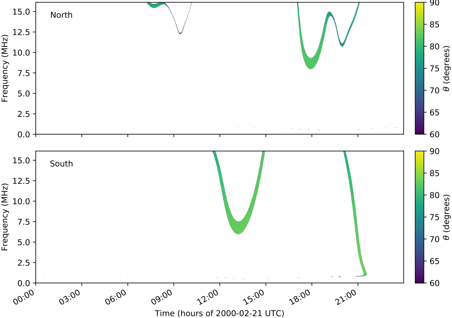
expres_cassini_jupiter_ganymede_isaac_lossc-wid1deg_3kev_20000221_v01.cdf
