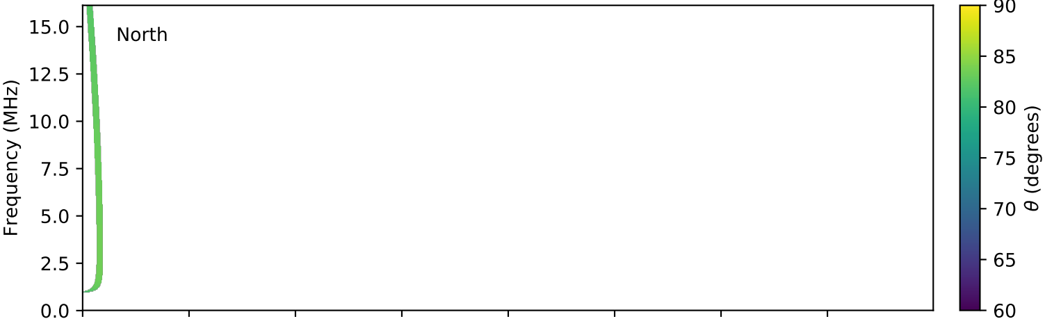
expres_cassini_jupiter_ganymede_isaac_lossc-wid1deg_3kev_20000215_v01.cdf
