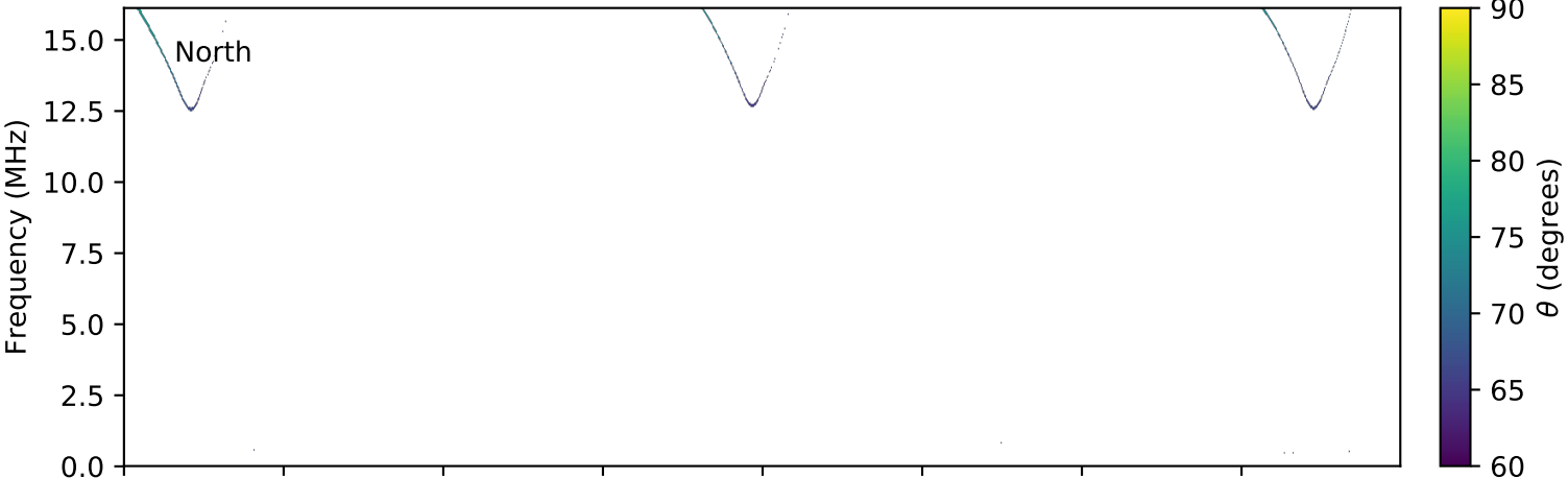
expres_cassini_jupiter_ganymede_isaac_lossc-wid1deg_3kev_20000213_v01.cdf
