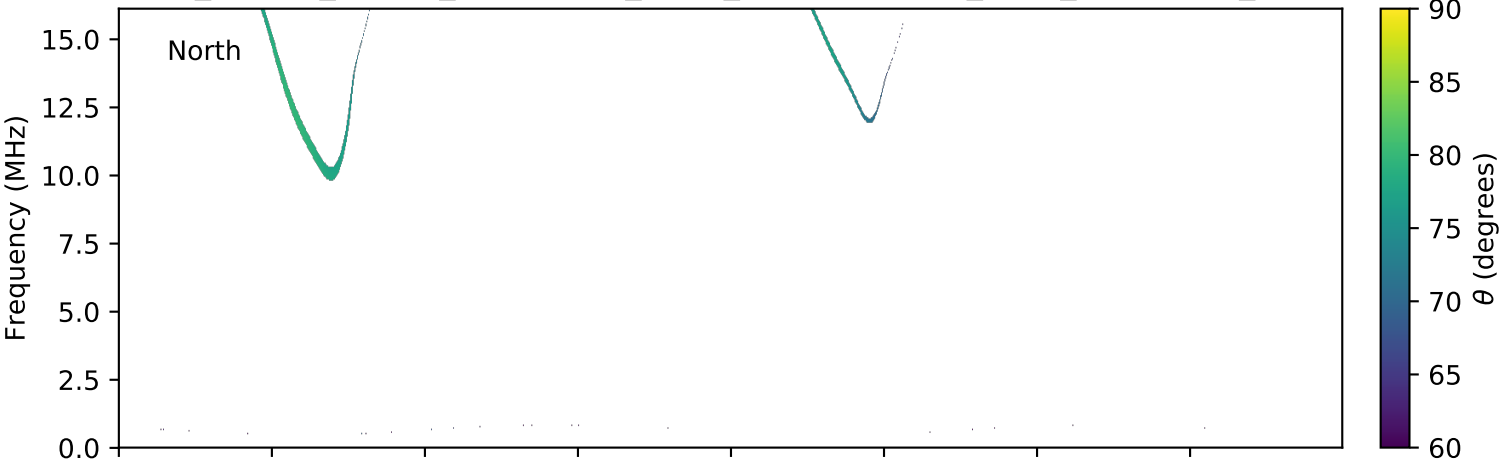
expres_cassini_jupiter_ganymede_isaac_lossc-wid1deg_3kev_20000212_v01.cdf
