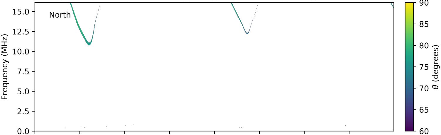
expres_cassini_jupiter_ganymede_isaac_lossc-wid1deg_3kev_20000205_v01.cdf
