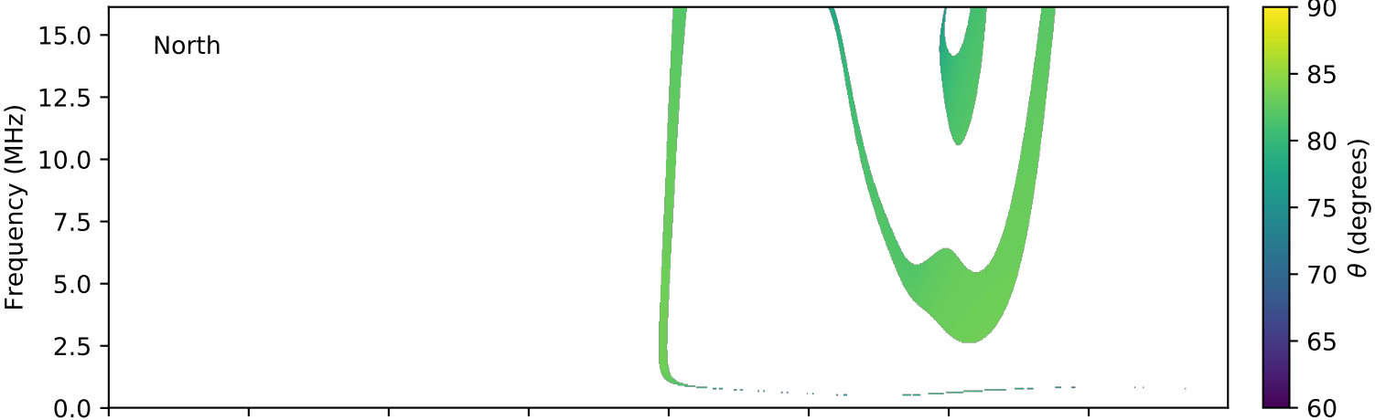
expres_cassini_jupiter_ganymede_isaac_lossc-wid1deg_3kev_20000204_v01.cdf
