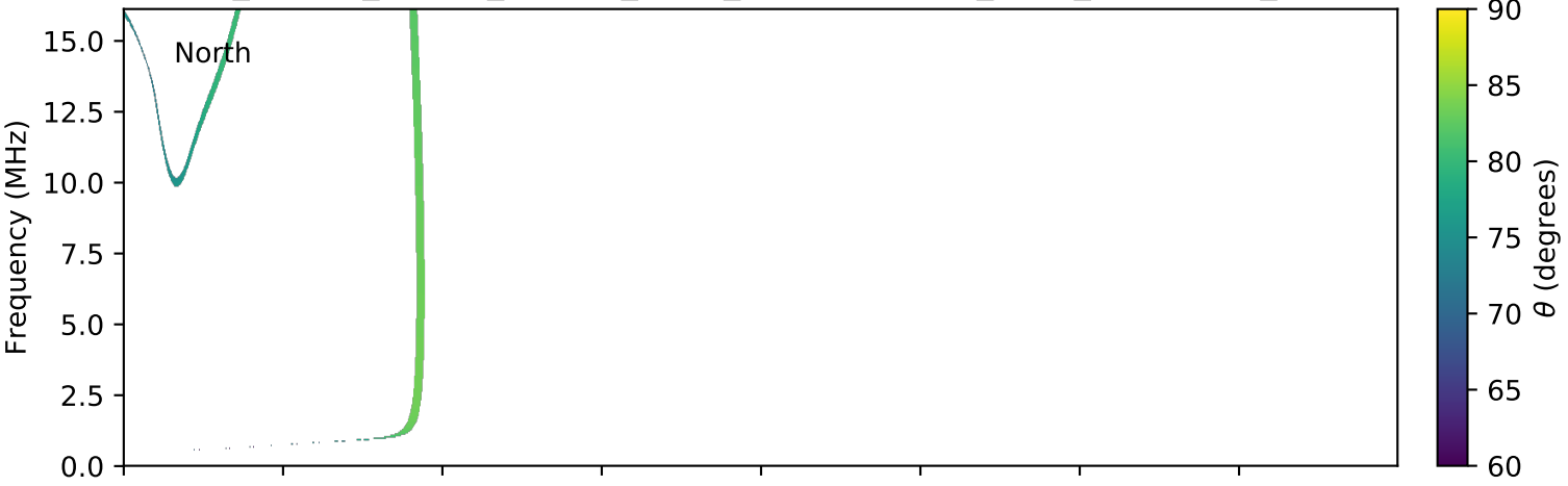
expres_cassini_jupiter_europa_isaac_lossc-wid1deg_3kev_20000228_v01.cdf
