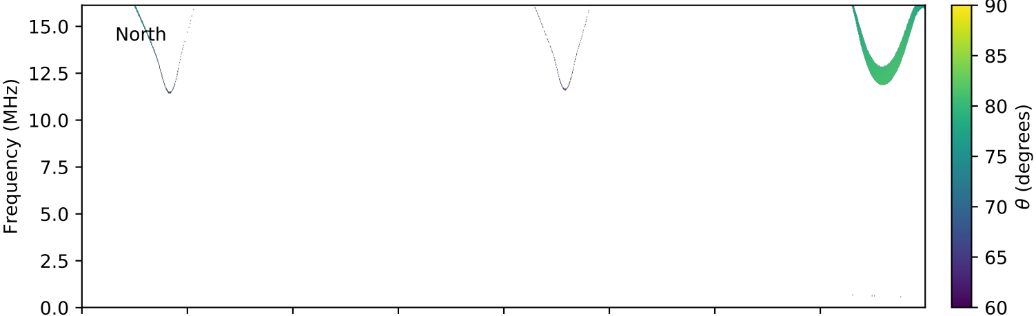
expres_cassini_jupiter_europa_isaac_lossc-wid1deg_3kev_20000227_v01.cdf
