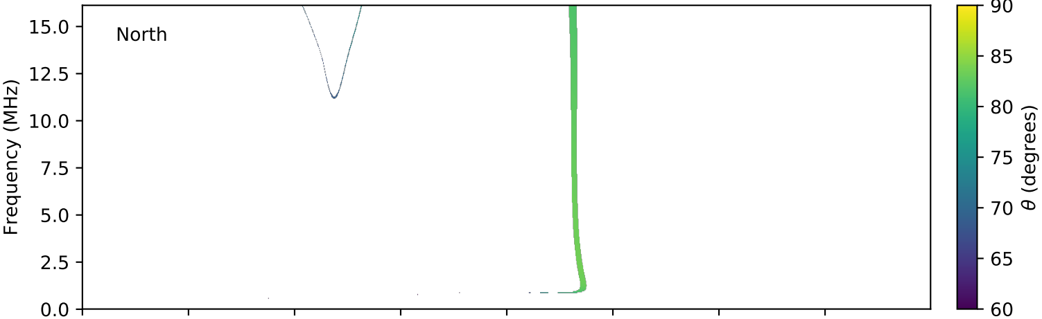
expres_cassini_jupiter_europa_isaac_lossc-wid1deg_3kev_20000224_v01.cdf
