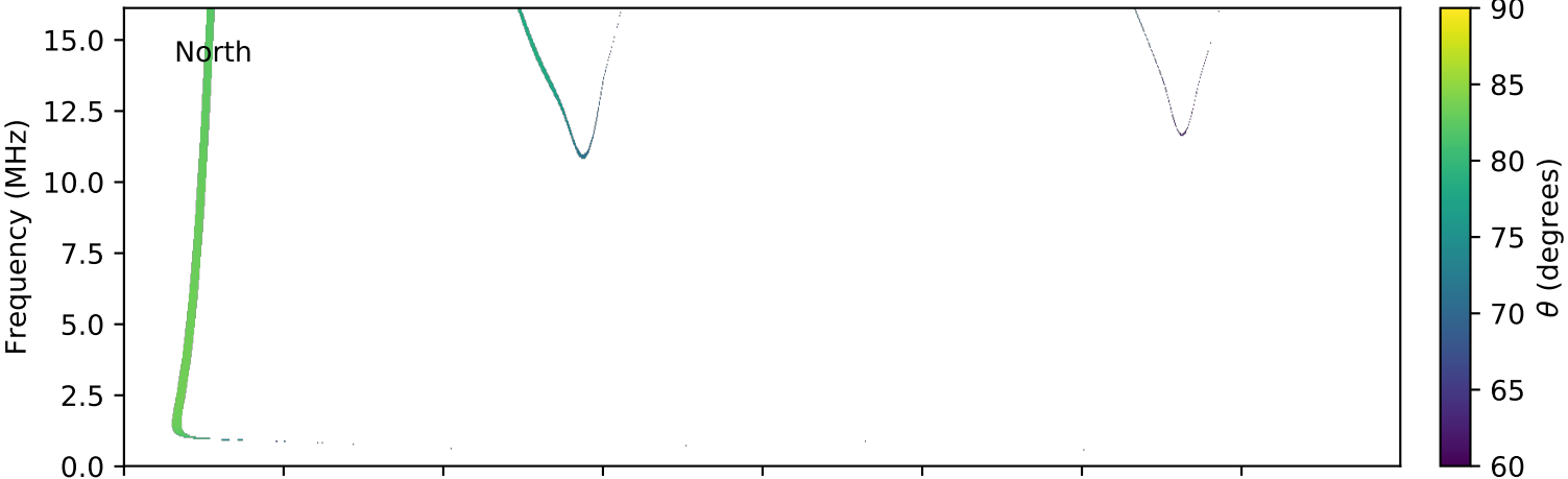
expres_cassini_jupiter_europa_isaac_lossc-wid1deg_3kev_20000223_v01.cdf
