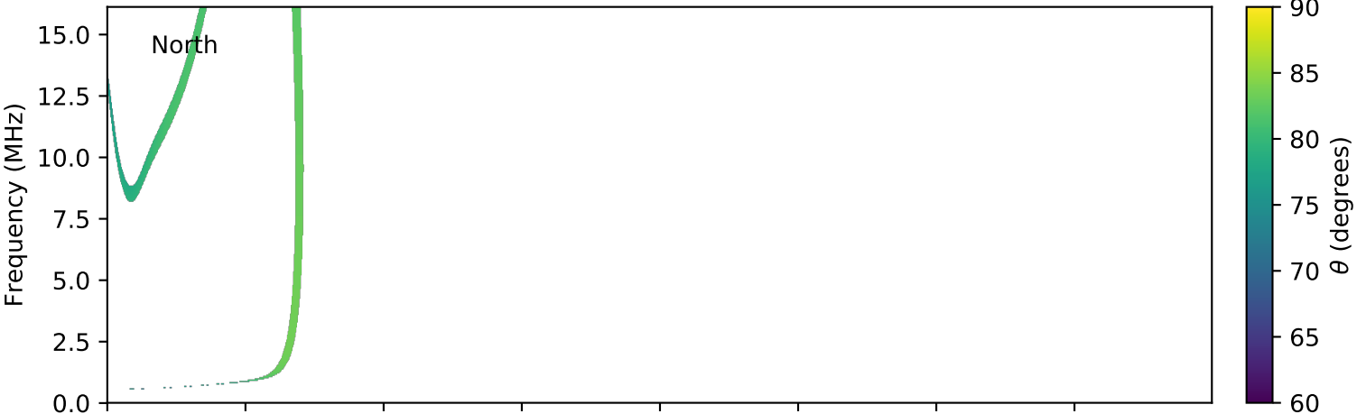
expres_cassini_jupiter_europa_isaac_lossc-wid1deg_3kev_20000221_v01.cdf
