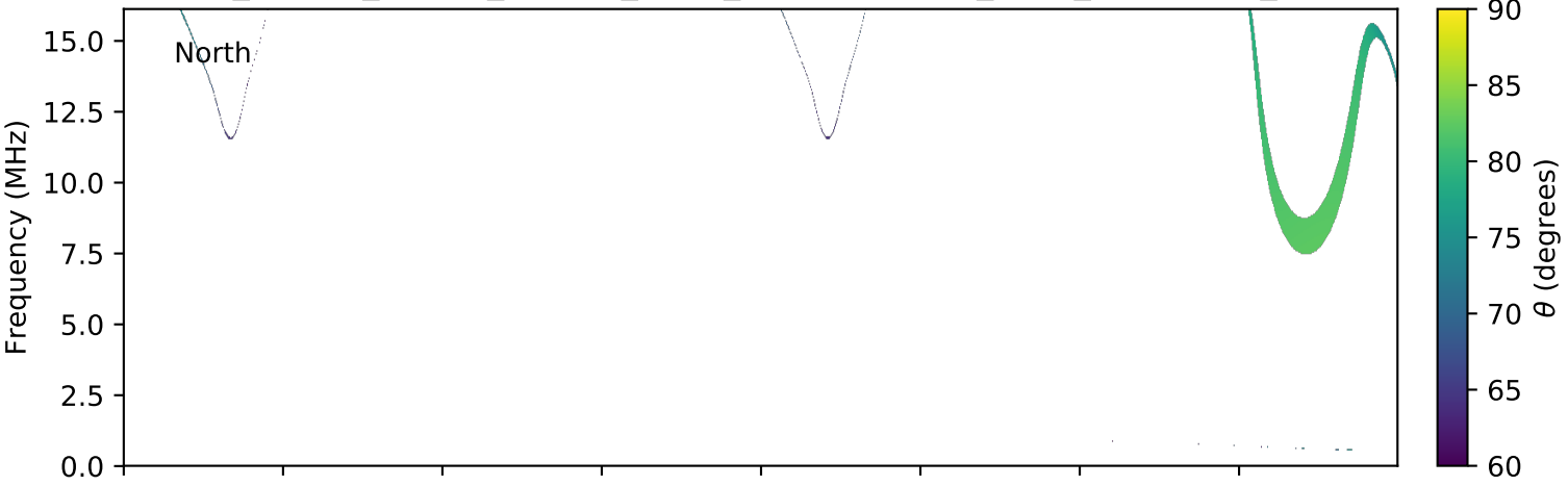
expres_cassini_jupiter_europa_isaac_lossc-wid1deg_3kev_20000220_v01.cdf
