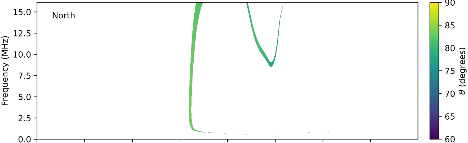
expres_cassini_jupiter_europa_isaac_lossc-wid1deg_3kev_20000219_v01.cdf
