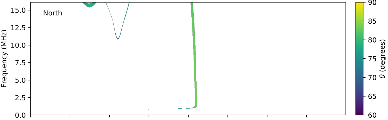
expres_cassini_jupiter_europa_isaac_lossc-wid1deg_3kev_20000217_v01.cdf
