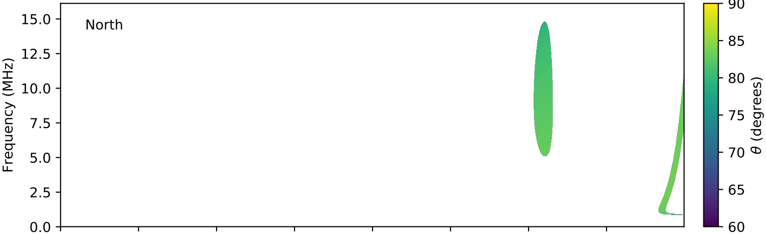
expres_cassini_jupiter_europa_isaac_lossc-wid1deg_3kev_20000215_v01.cdf
