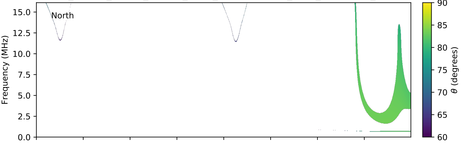
expres_cassini_jupiter_europa_isaac_lossc-wid1deg_3kev_20000213_v01.cdf
