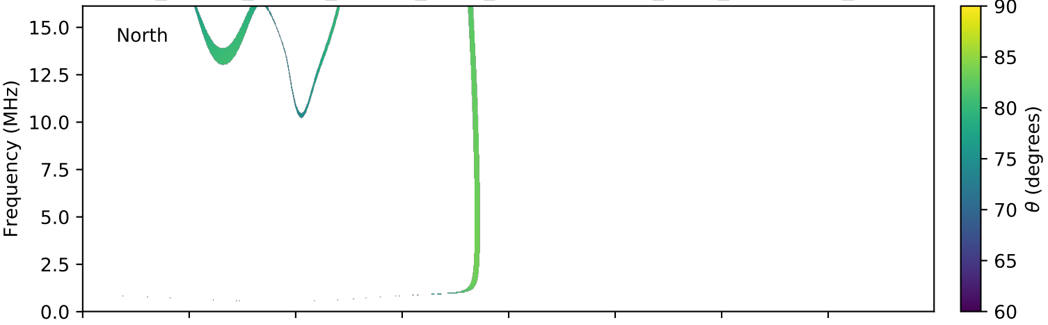
expres_cassini_jupiter_europa_isaac_lossc-wid1deg_3kev_20000210_v01.cdf
