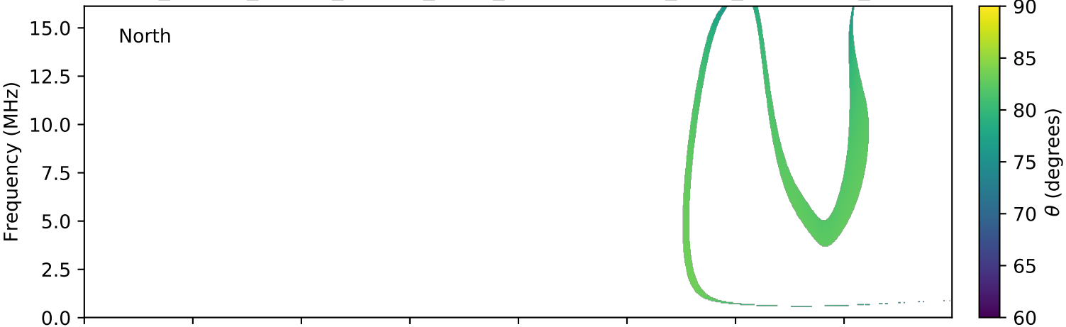
expres_cassini_jupiter_europa_isaac_lossc-wid1deg_3kev_20000208_v01.cdf
