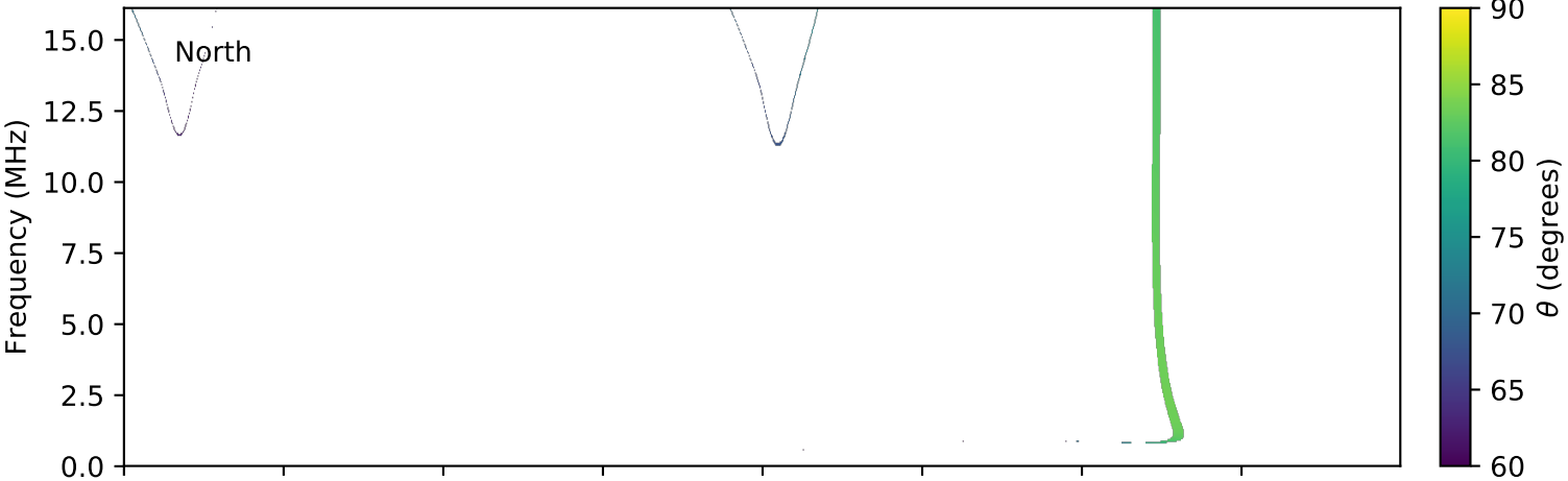
expres_cassini_jupiter_europa_isaac_lossc-wid1deg_3kev_20000206_v01.cdf
