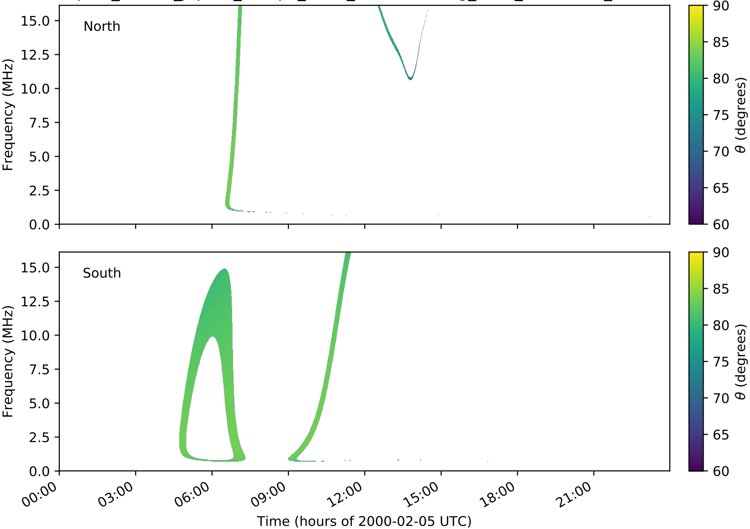
expres_cassini_jupiter_europa_isaac_lossc-wid1deg_3kev_20000205_v01.cdf
