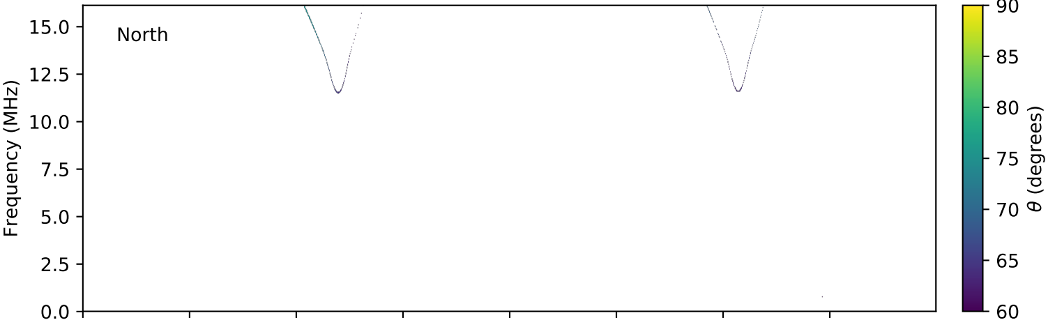
expres_cassini_jupiter_europa_isaac_lossc-wid1deg_3kev_20000202_v01.cdf
