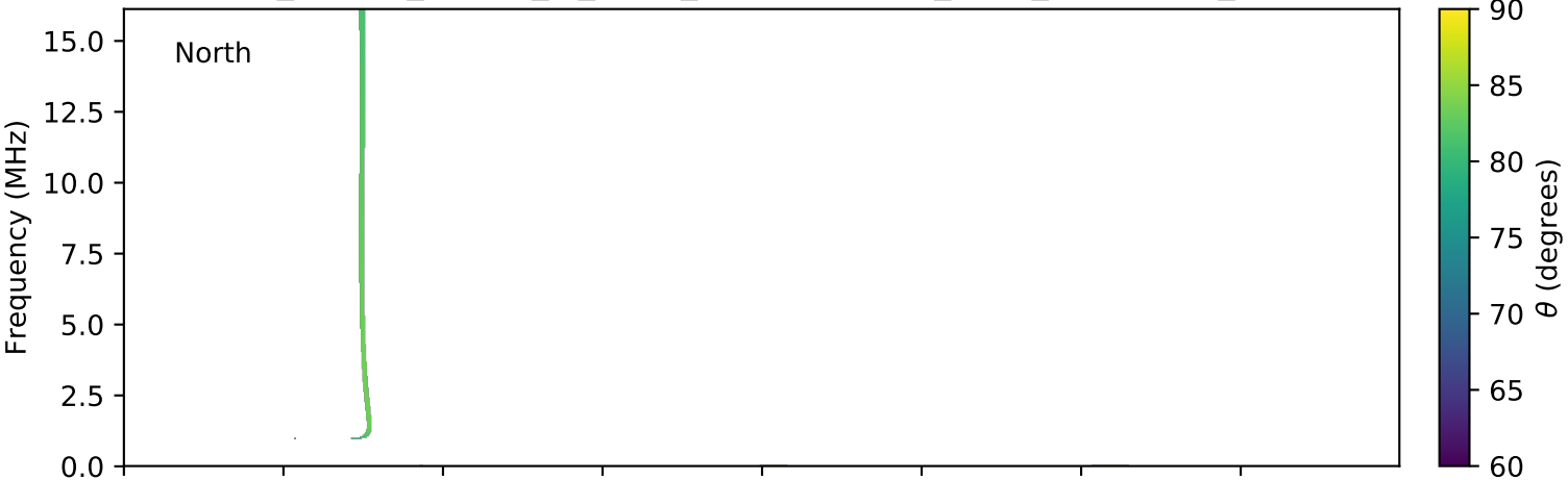
expres_cassini_jupiter_io_isaac_lossc-wid1deg_3kev_20000131_v01.cdf
