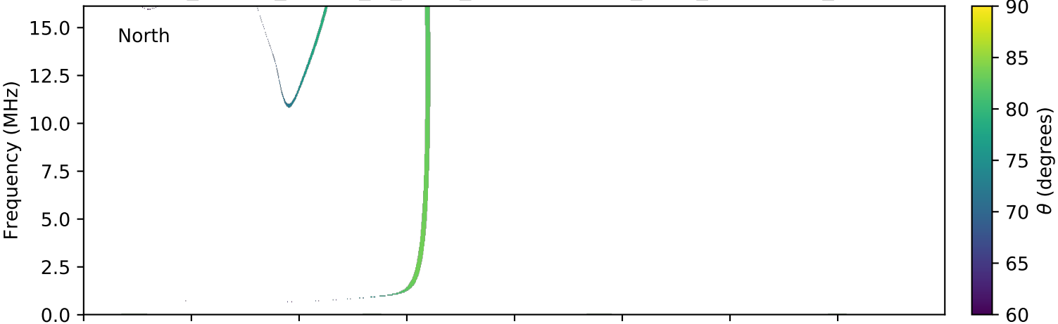
expres_cassini_jupiter_io_isaac_lossc-wid1deg_3kev_20000122_v01.cdf
