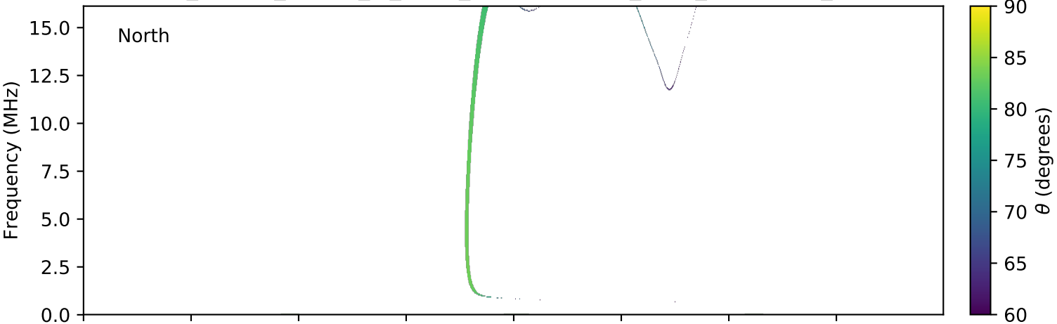
expres_cassini_jupiter_io_isaac_lossc-wid1deg_3kev_20000114_v01.cdf
